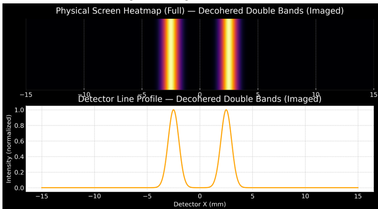
Figure 4 — Imaged detector (full).
