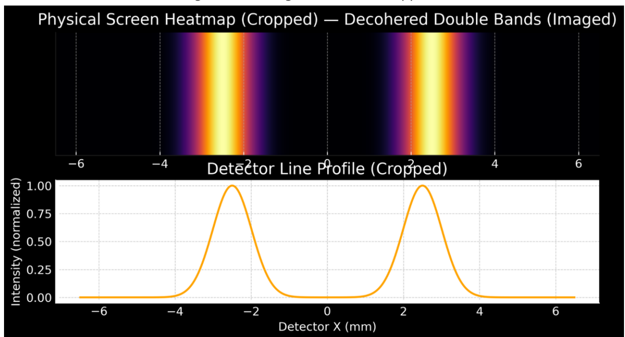
Figure 5 — Imaged detector (cropped).
