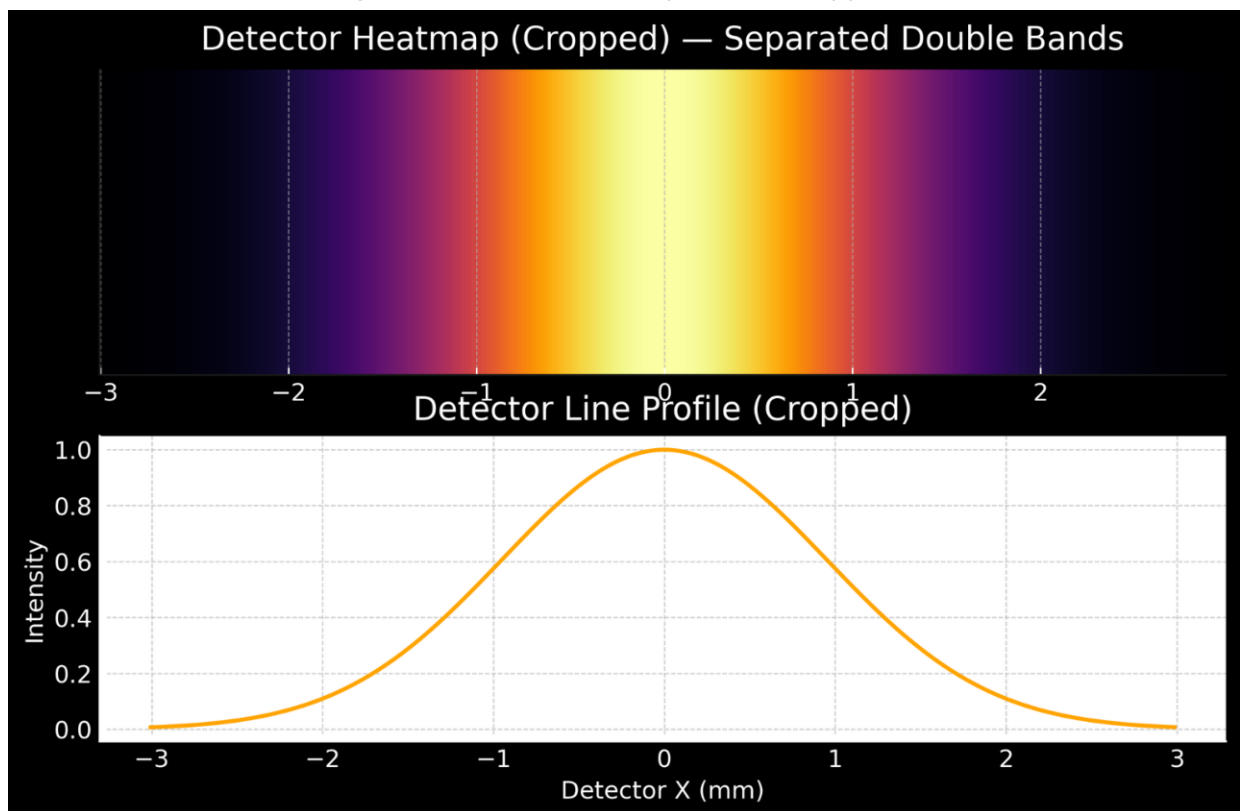
Figure 9 — Fraunhofer separated (cropped).
